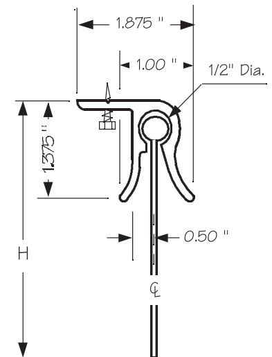
HEAVY DUTY IN JAMB BONDED BEAD
