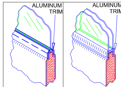
SINGLE PANE DOUBLE PANE
