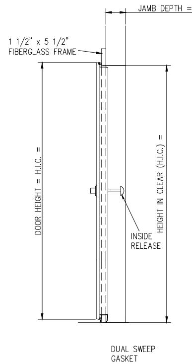
SIDE VIEW SECTION
